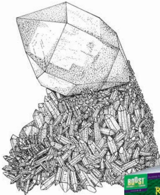
Amethyst (North Carolina) CC: Silicon dioxide. H: 7. SG: 2.6. Cr: Hexagonal. Amethyst is a variety of quartz that is purple or "amethyst" in color, the result of traces of manganese. This single amethyst crystal occurred as a secondary growth on a plate of clear quartz crystals. It was in the several amethyst mines in North Carolina. Amethyst is the more select crystal gemstones.
